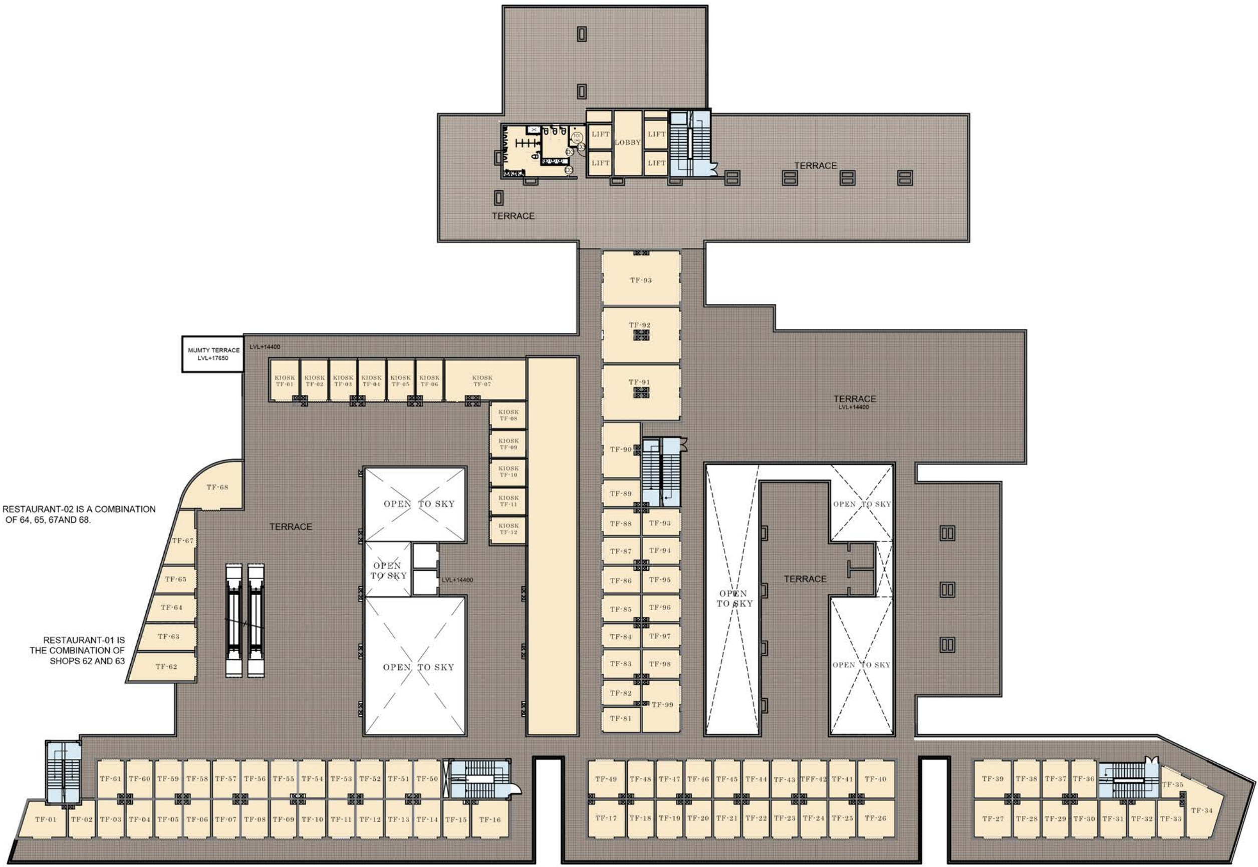
THIRD FLOOR PLAN (BLOCK A)
